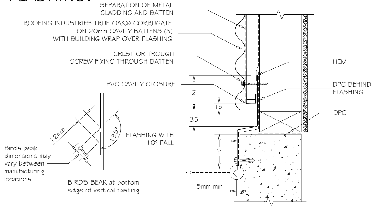
HORIZONTAL CLADDING JUNCTION 1:5
