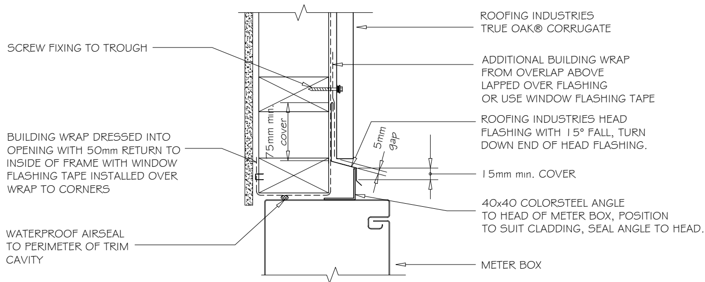
METER BOX HEAD FLASHING VERTICAL TRUE OAK® CORRUGATED 1:5
