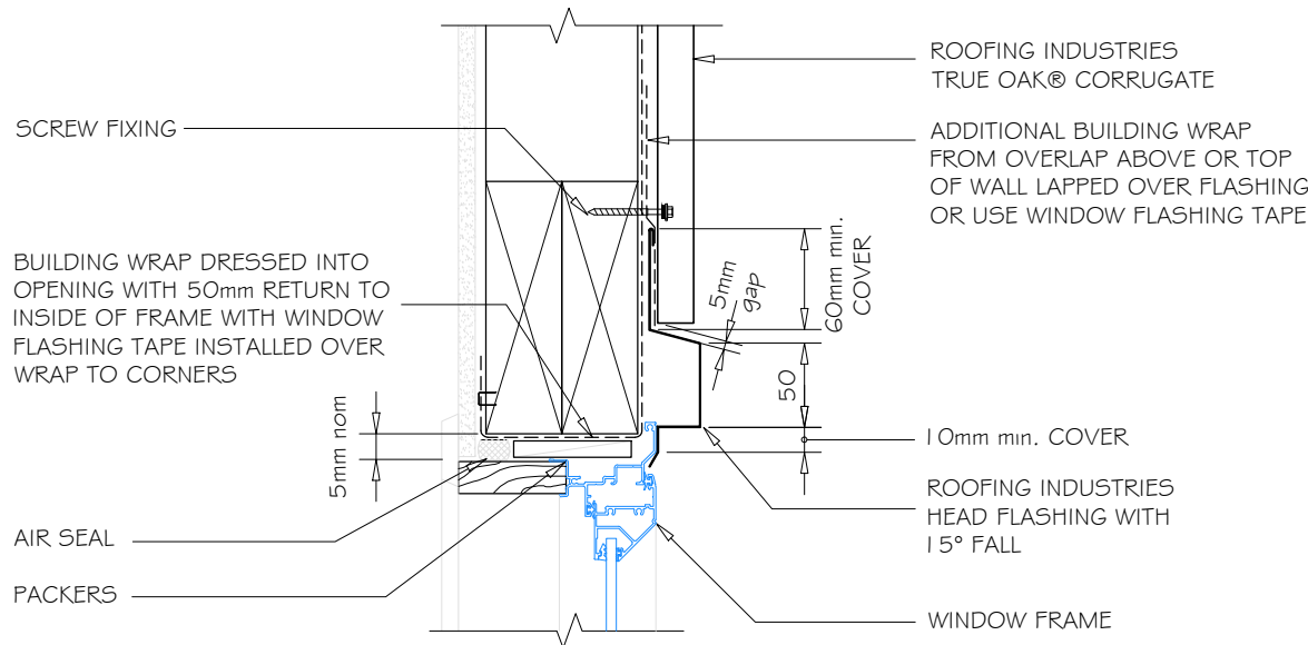
WINDOW HEAD VERTICAL TRUE OAK® CORRUGATE 1:5
