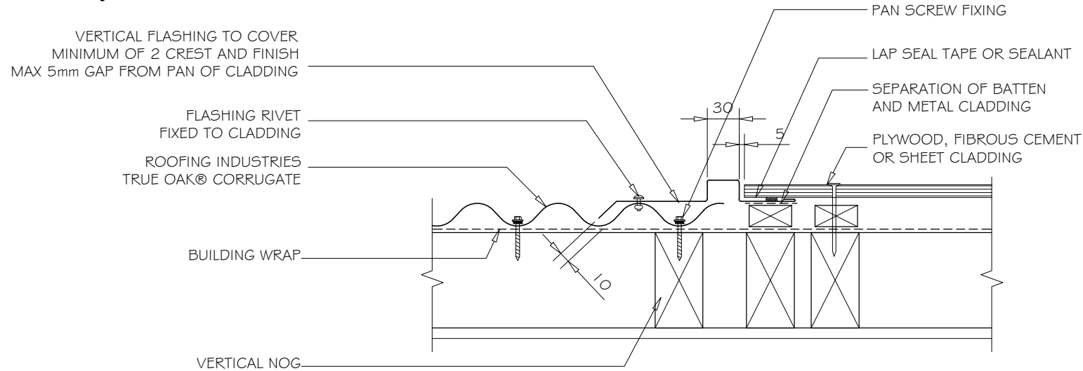
VERTICAL BUTT FLASHING - CLADDING CHANGE 1:5
