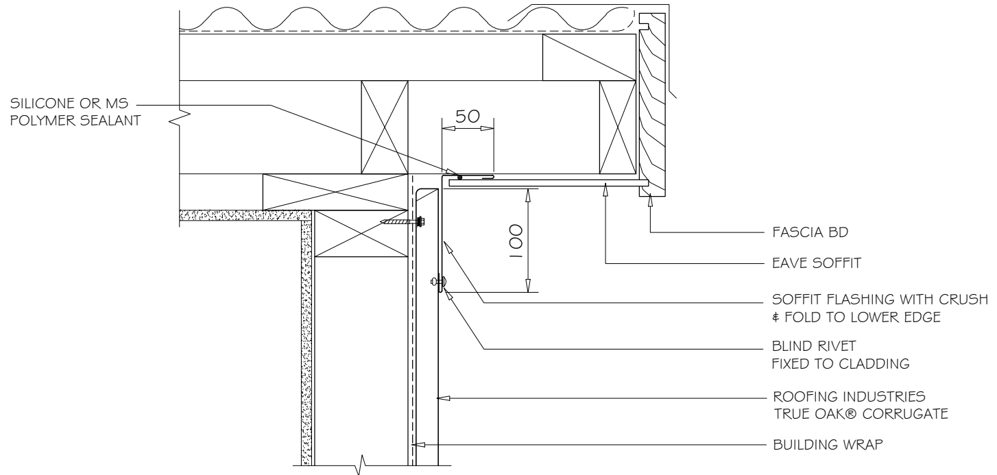
SOFFIT FLASHING 1:5
