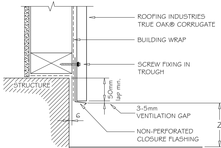
BOTTOM OF CLADDING PROFILE 1:5
