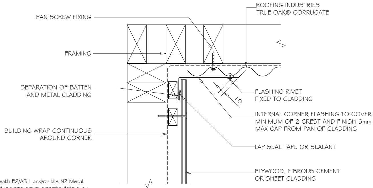
INTERNAL CORNER PROFILE 1:5
