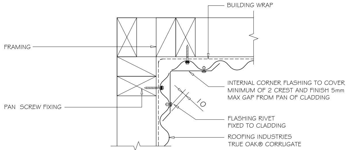
INTERNAL CORNER PROFILE 1:5
