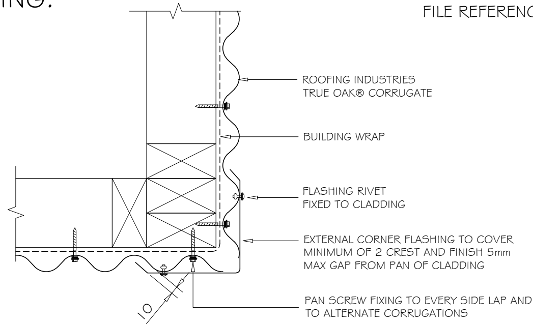
EXTERNAL CORNER PROFILE 1:5
