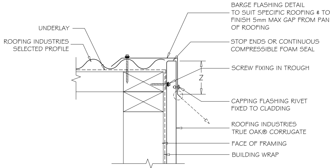
BARGE DETAIL VERTICAL CLADDING (KICK-OUT) 1:5
