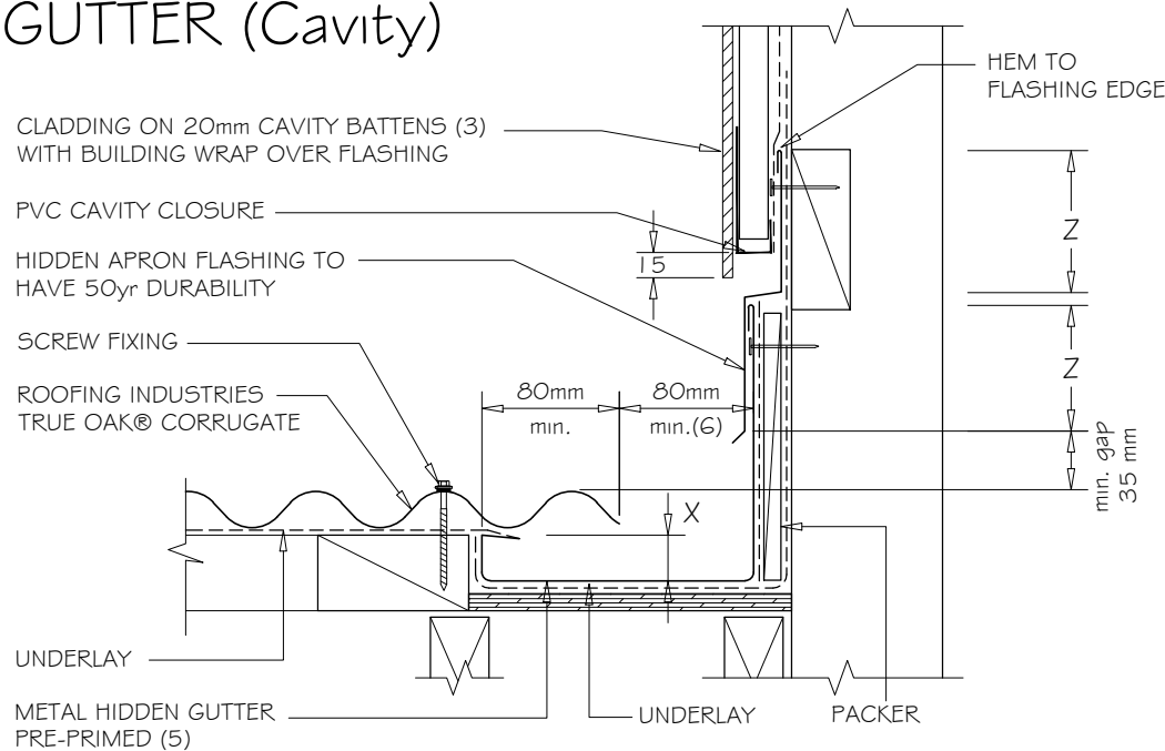
PARALLEL HIDDEN or OBTUSE 2 PIECE GUTTER PROFILE 1:5
