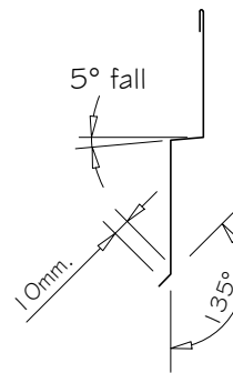
PARALLEL HIDDEN or OBTUSE 2 PIECE GUTTER PROFILE 1:5
