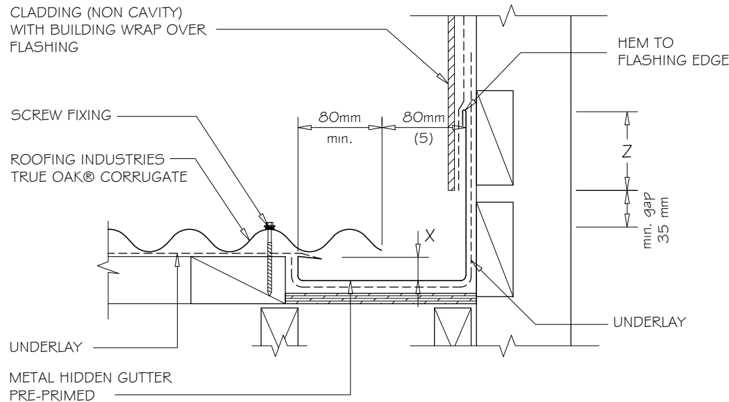
PARALLEL HIDDEN or OBTUSE GUTTER PROFILE 1:5
