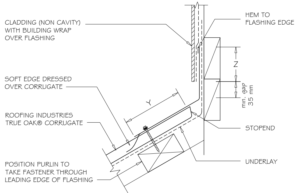
APRON FLASHING PROFILE 1:5
