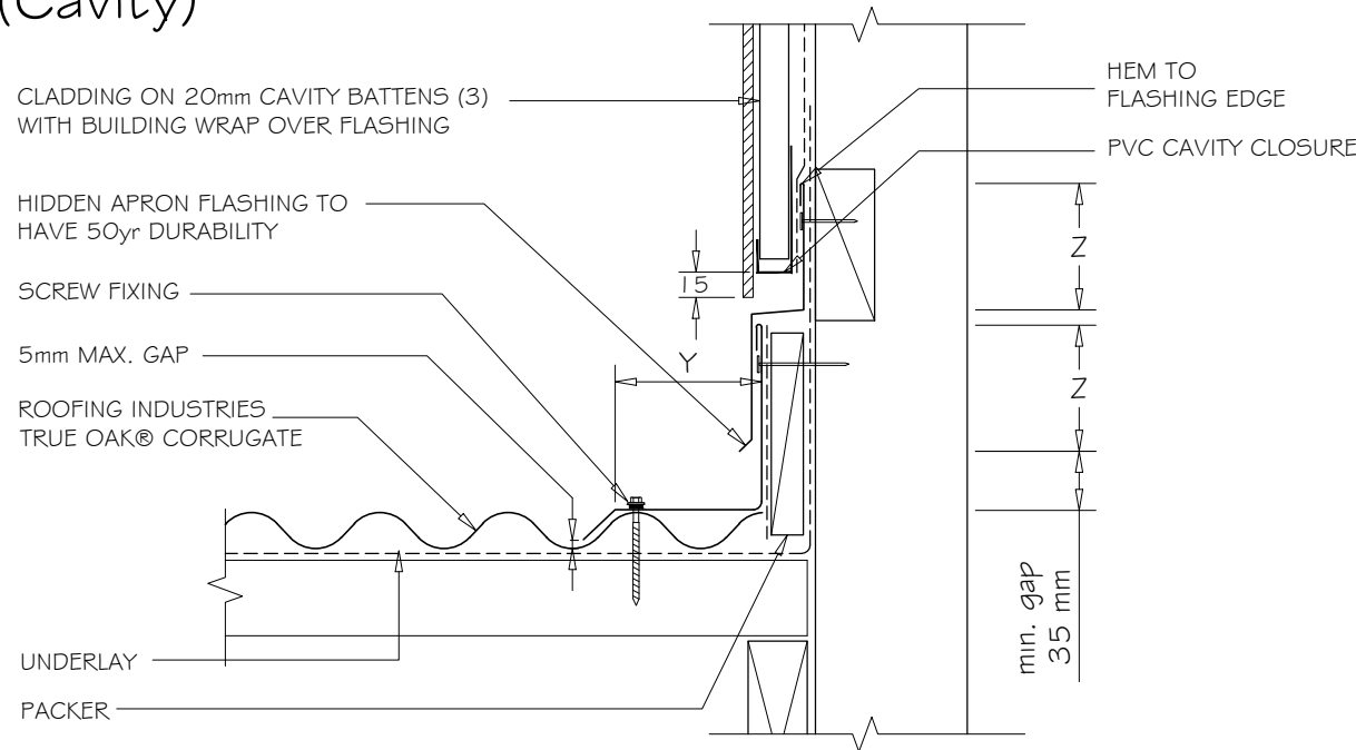
PARALLEL 2 PIECE APRON FLASHING 1:5
