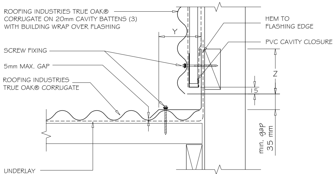
PARALLEL APRON FLASHING PROFILE 1:5
