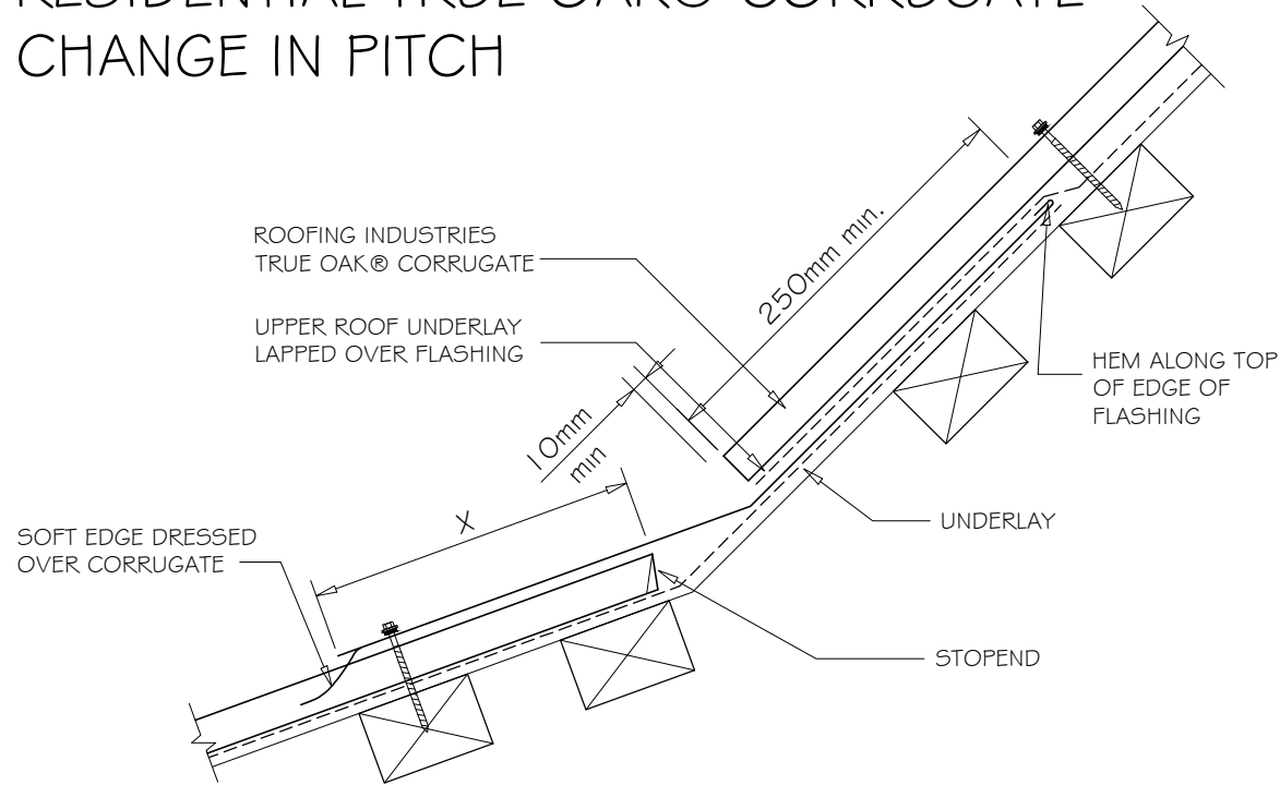
CHANGE IN PITCH TRUE OAK® CORRUGATED PROFILE 1:5
